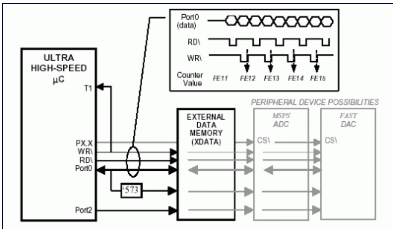
Figure 1. Hardware diagram for wr\ strobe counting.
